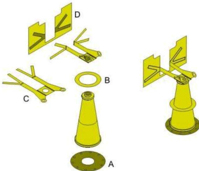
100G01 - 20mm Oerlikon Mk IIIA
